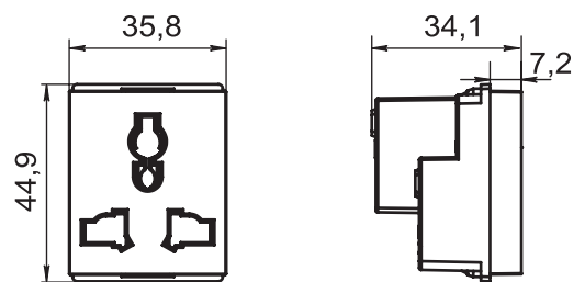
Socket 1/2 universal
